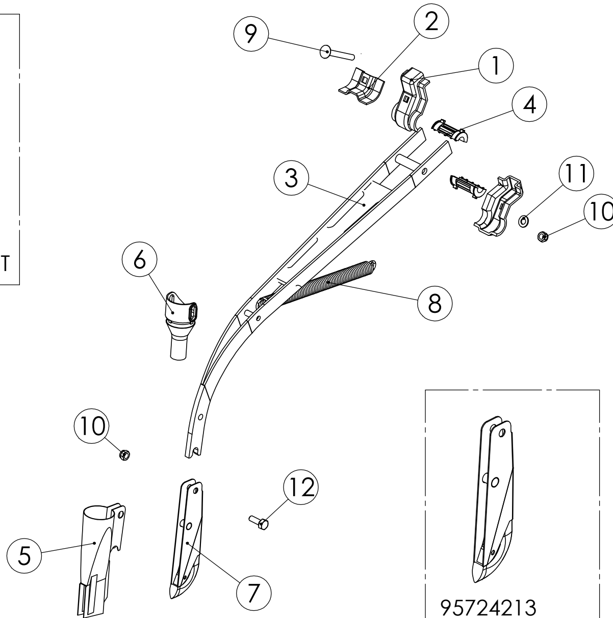
98840503 Suffolk coulter (Rear) Laahavannas (Taka)
