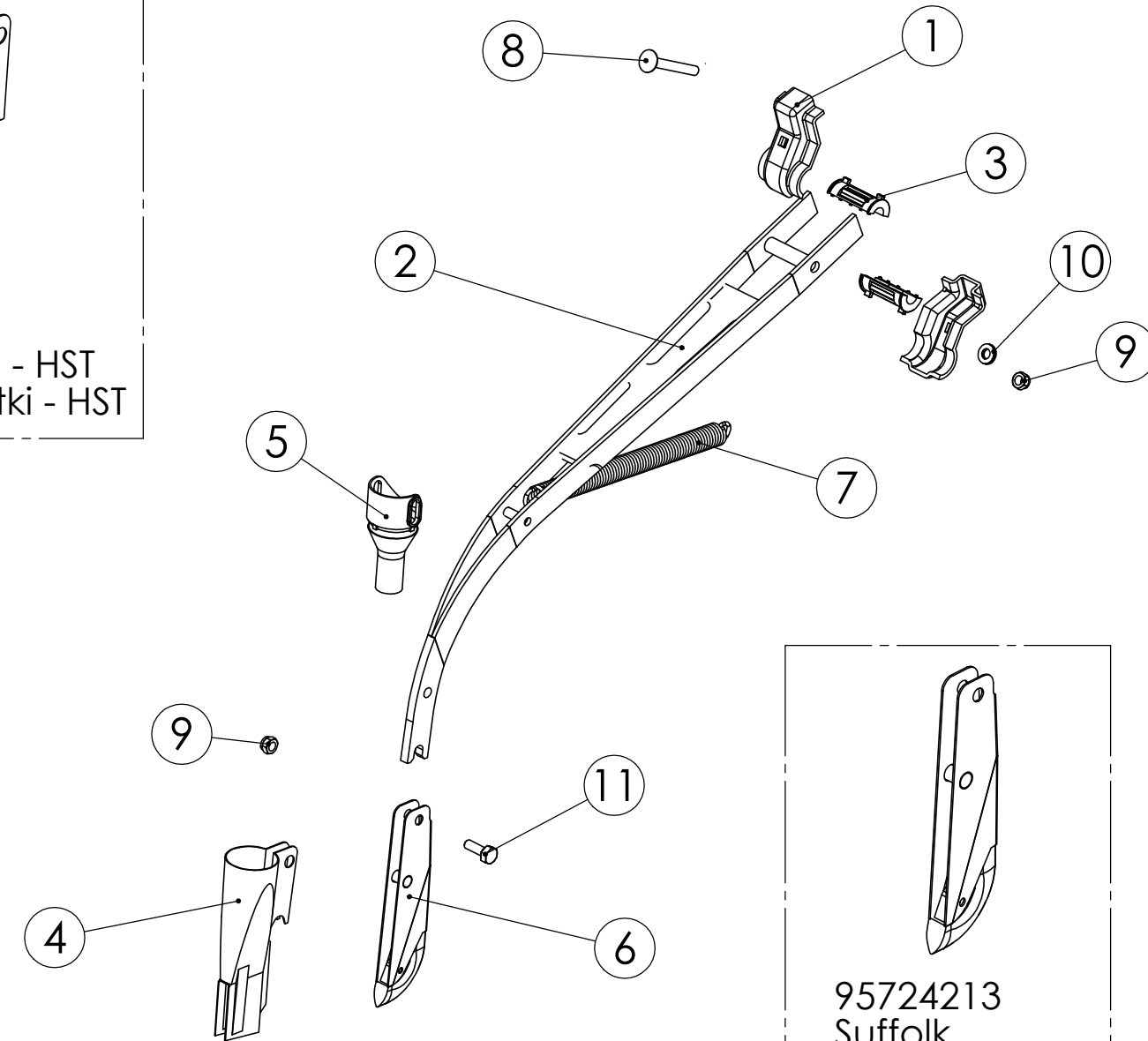
98840403 Suffolk coulter (Front) Laahavannas (Etu)
