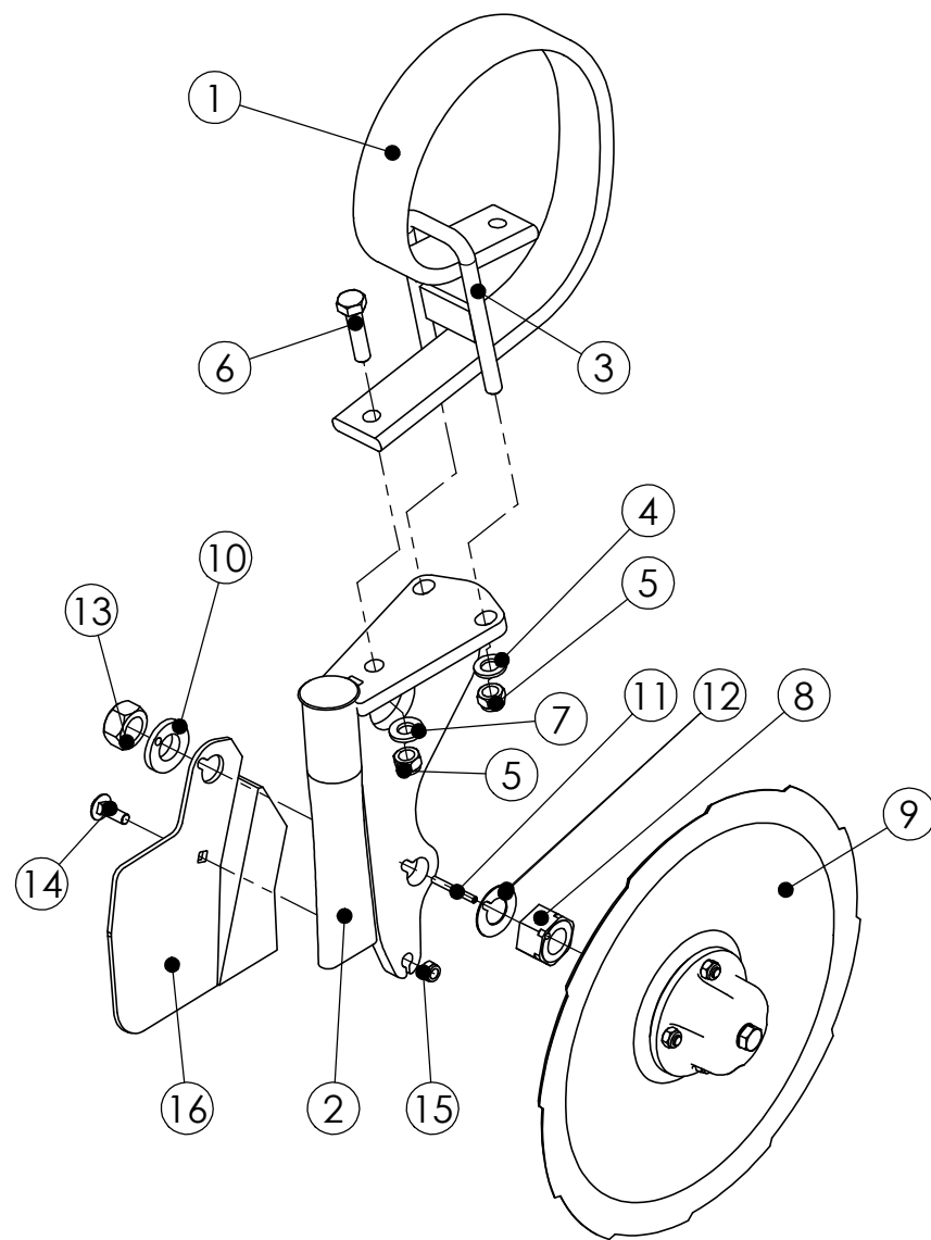
98853002 Laser coulter (Right) fertilizer Laservannas oikea lanfroite
