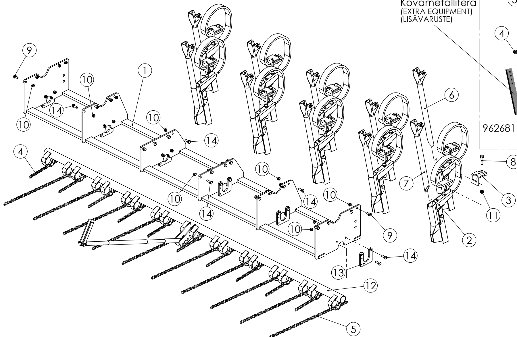
99199403 Frame for fertilizer coulters S-piikkirunko
