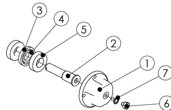
98853403 Axle + Hub Akseli + napa
