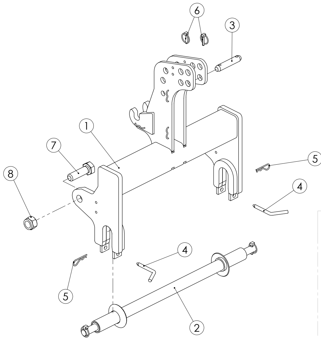
99192002 Drawbar Vetolaite
