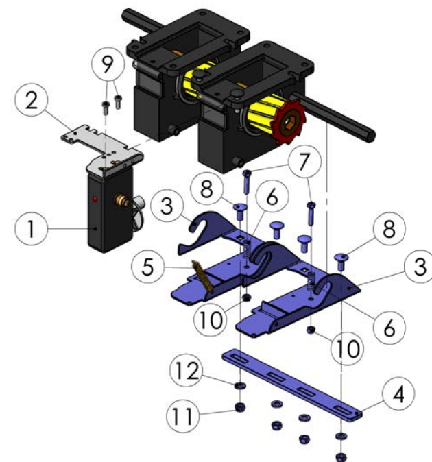
99012603 Stop motion, two feeding roller
