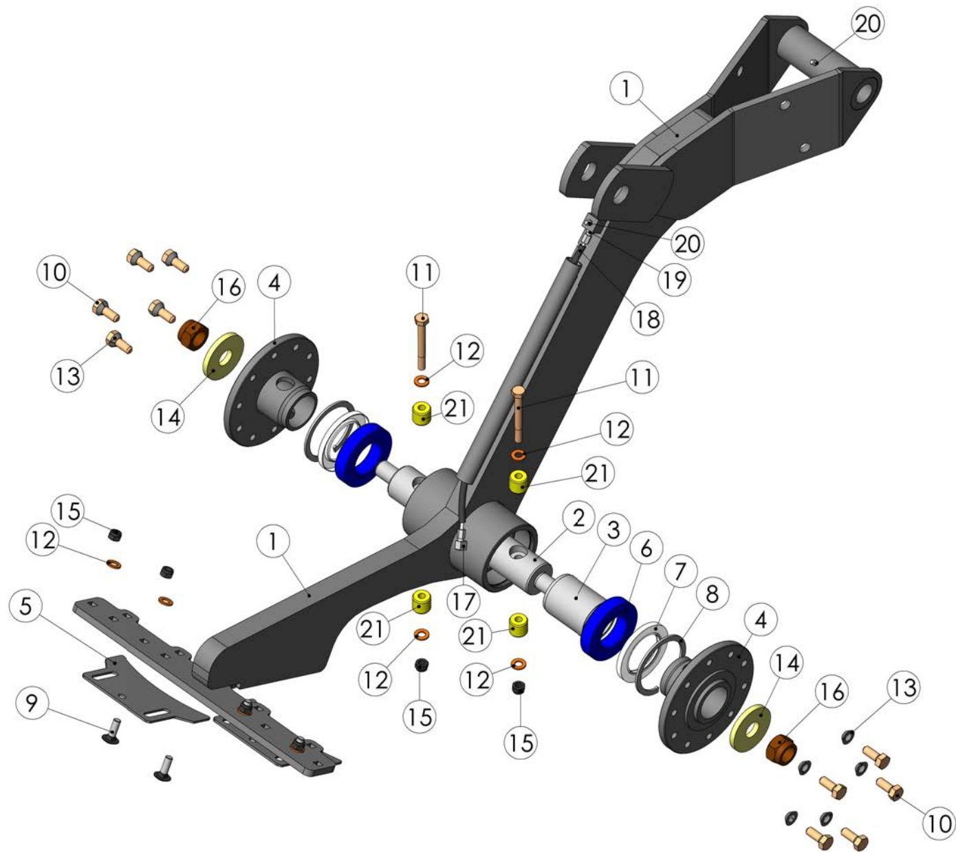
99496302 Support
