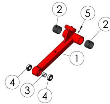
99296603 Front arm
