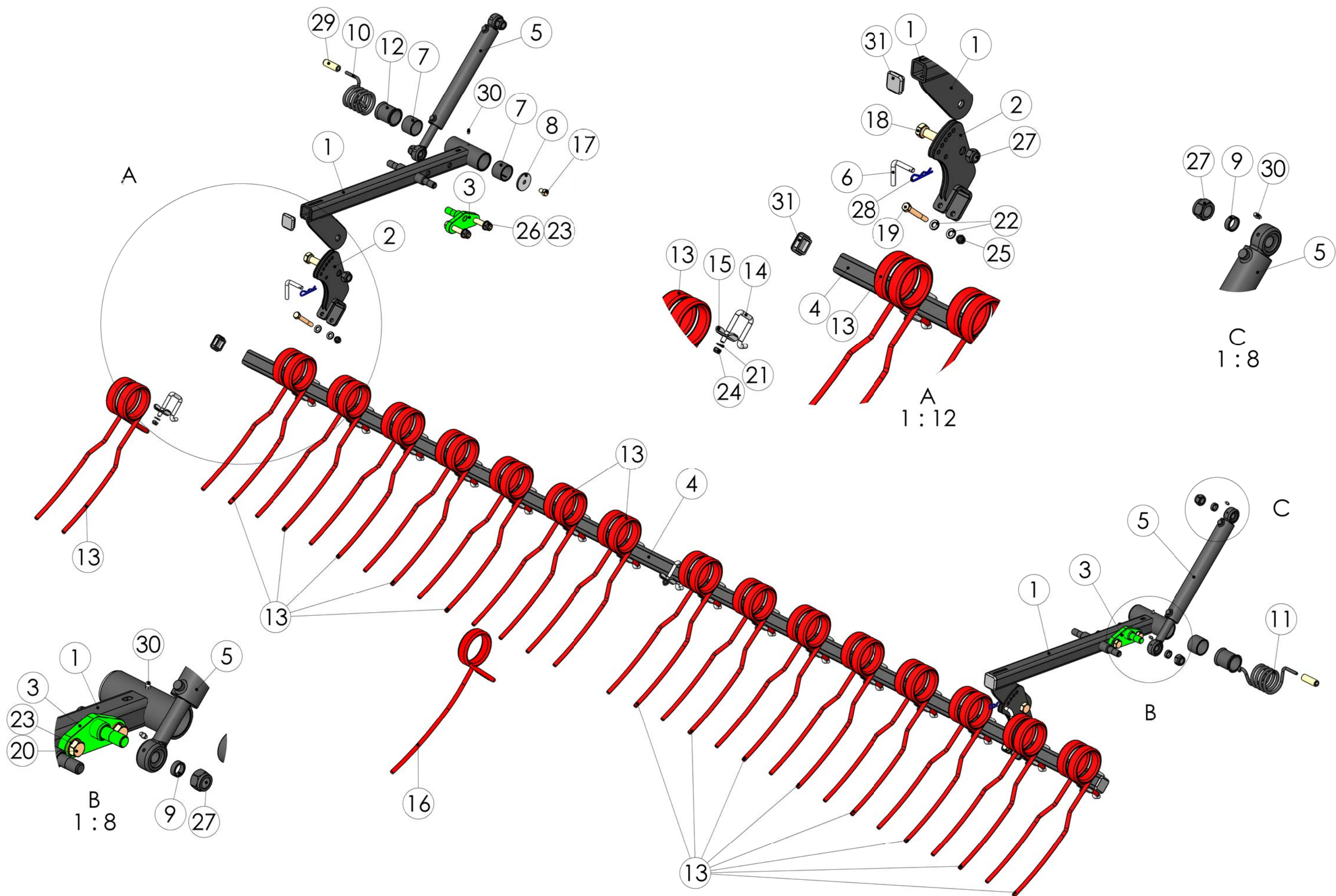
99525302 Rear harrow
