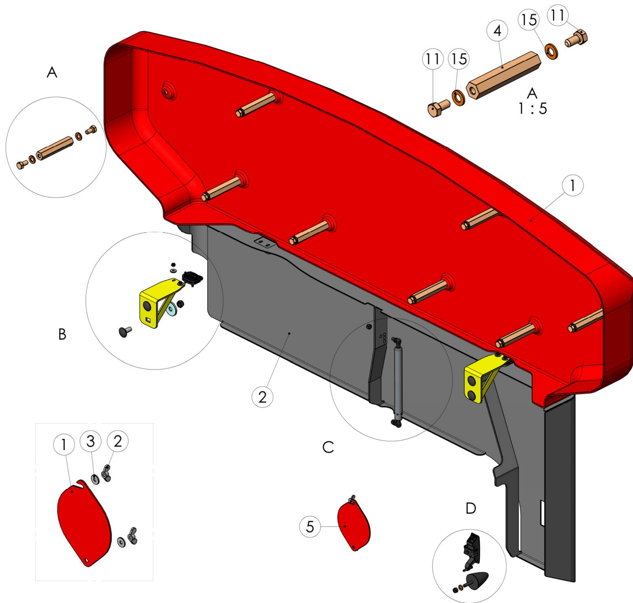
99503202 End cover left
