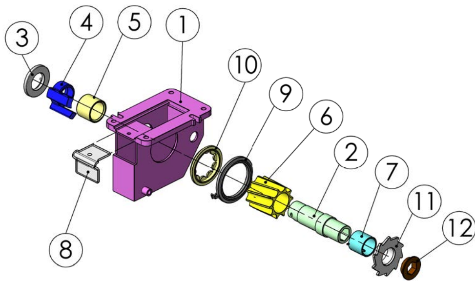
98453703 Tramline feeding chamber, fertilizer
