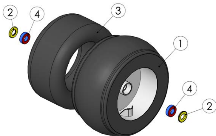
98162324 Tyre and rim
