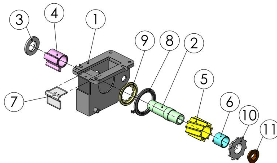
98453403 Tramline feeding chamber, seed
