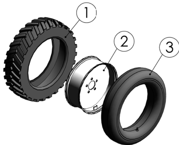
98725924 Tyre and rim left
