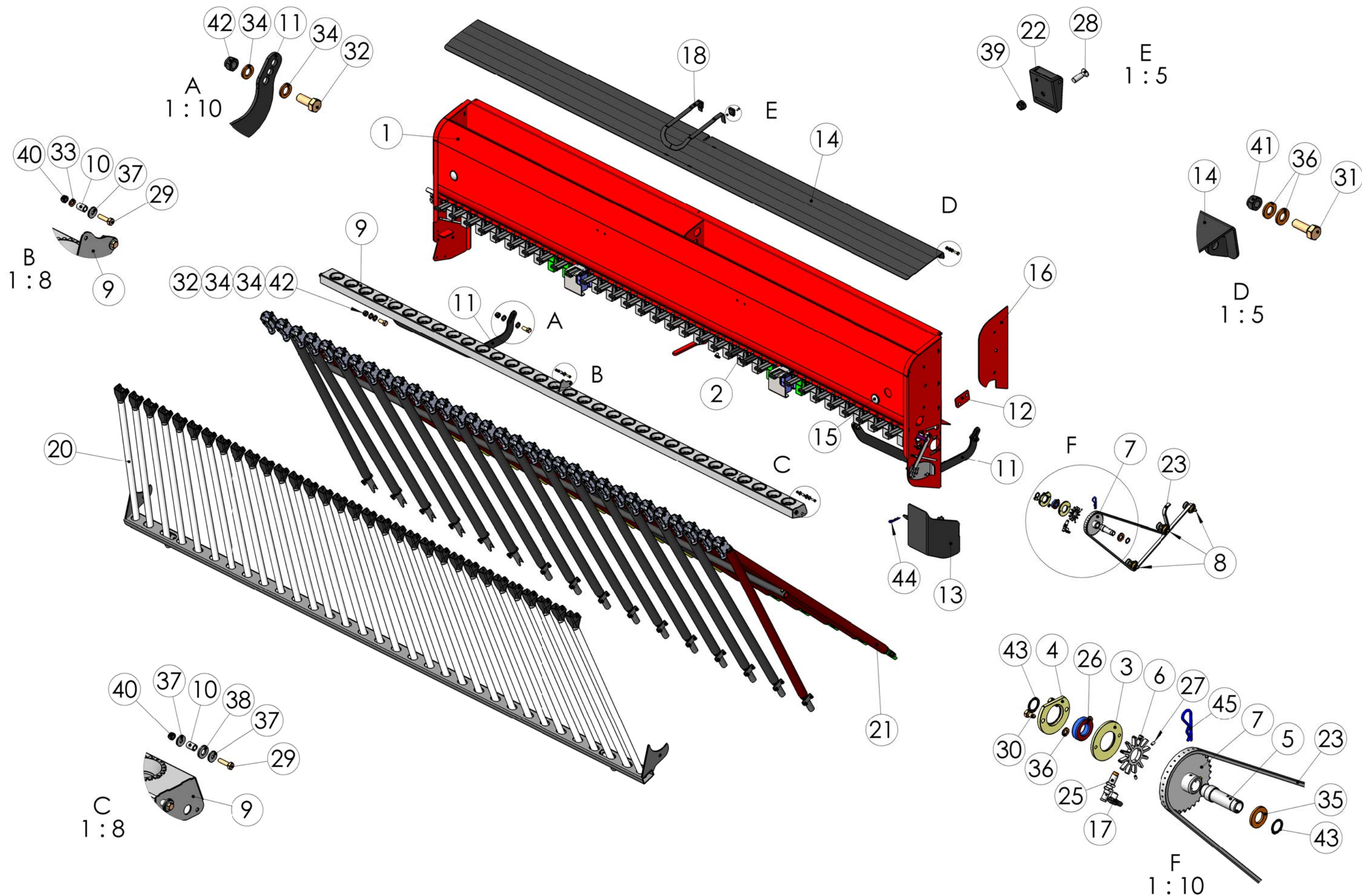
99525702 Grass seed drill
