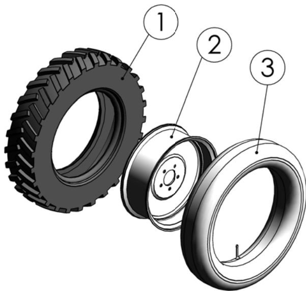
99300203 Tyre and rim left
