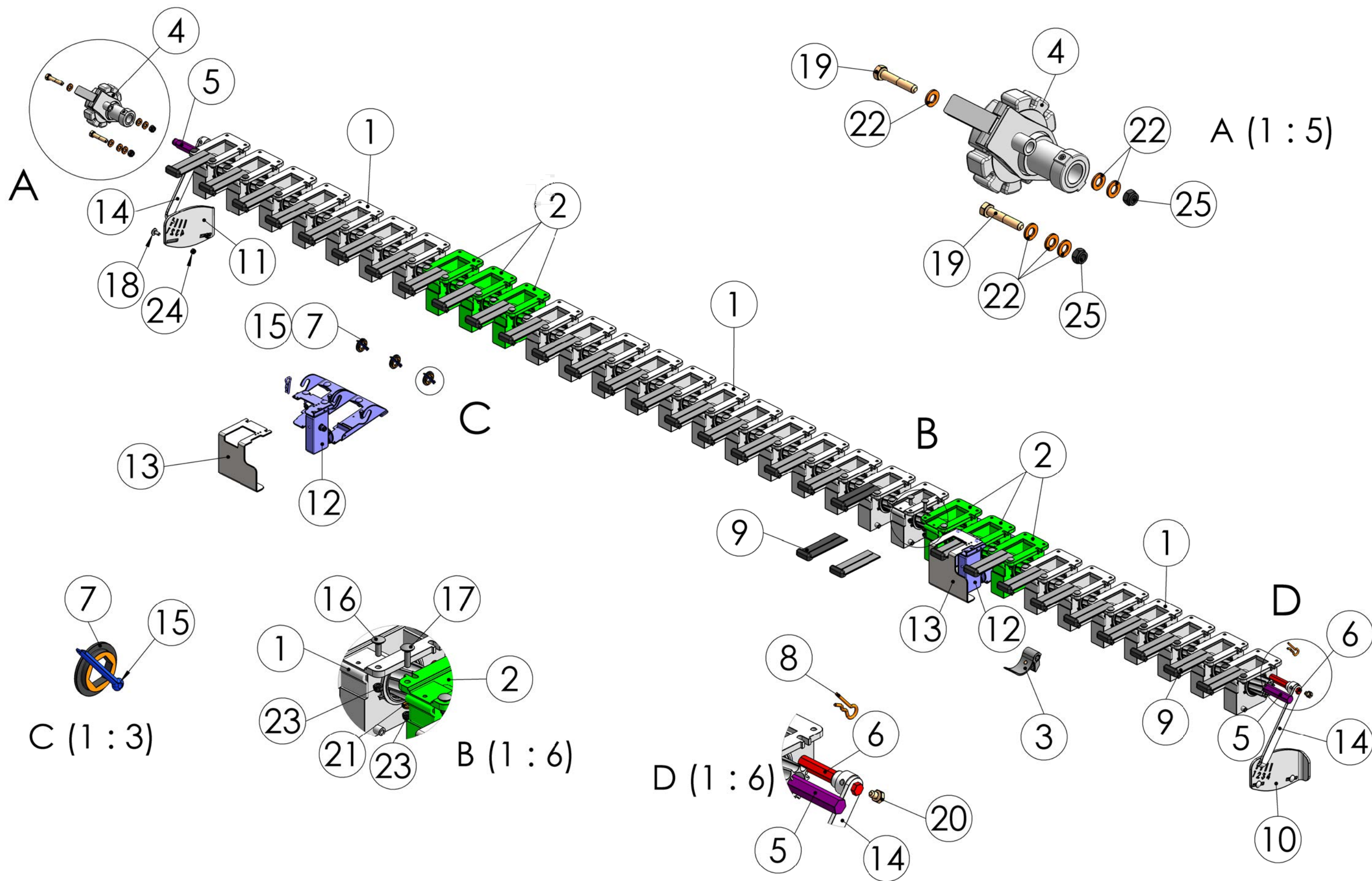
99530201 Feeding mechanism
