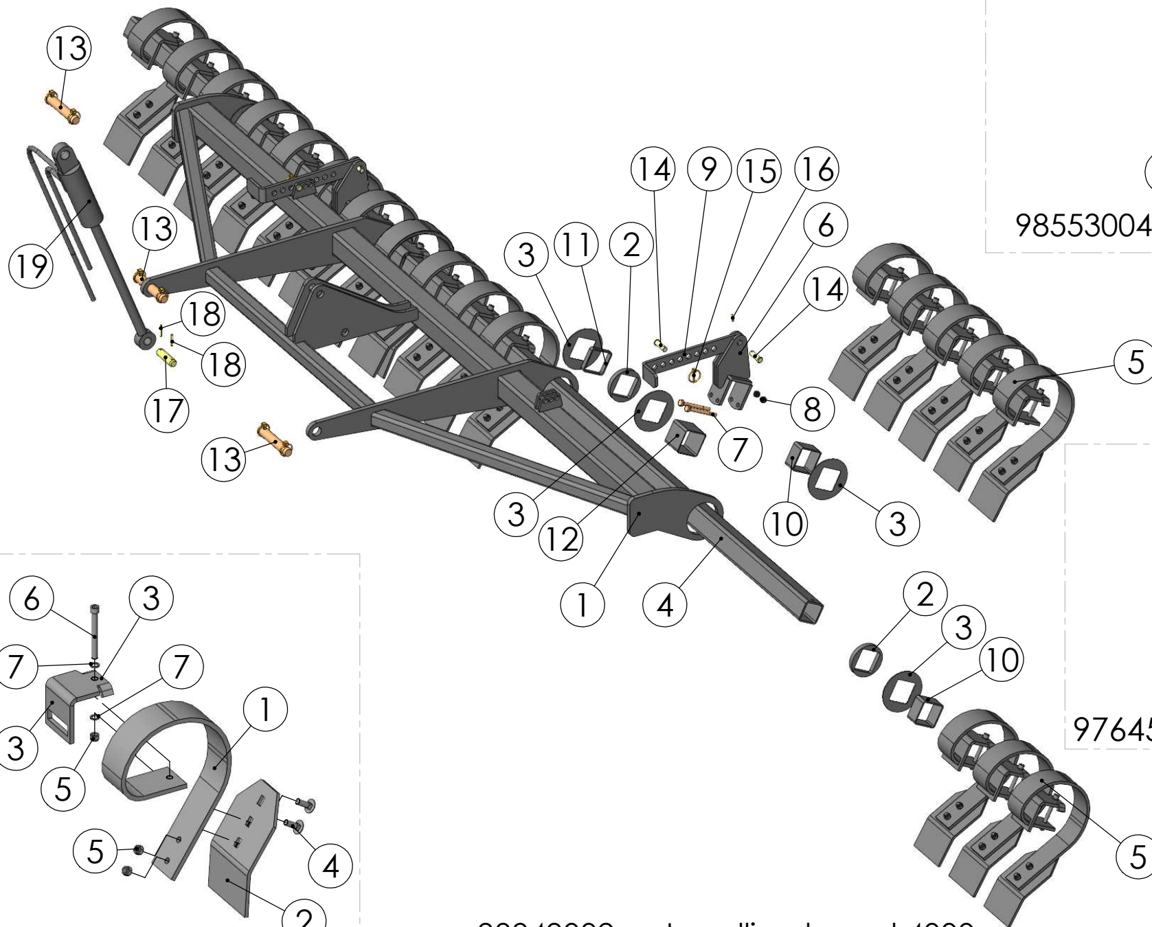
98849002 Levelling board 4000
