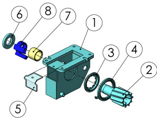
98314803 Feeding chamber, fertilizer
