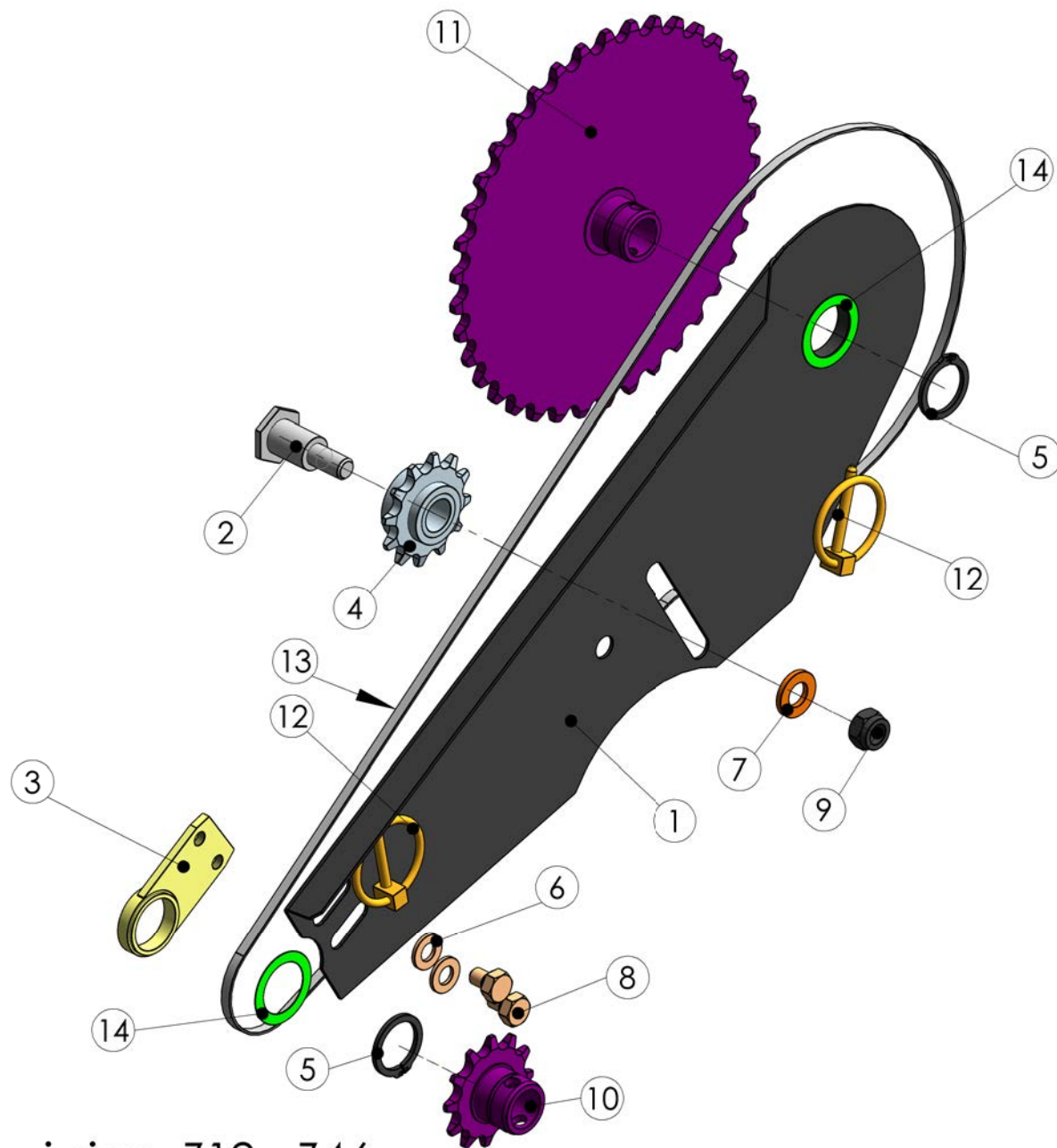
98836403 Transmission Z12 - Z46
