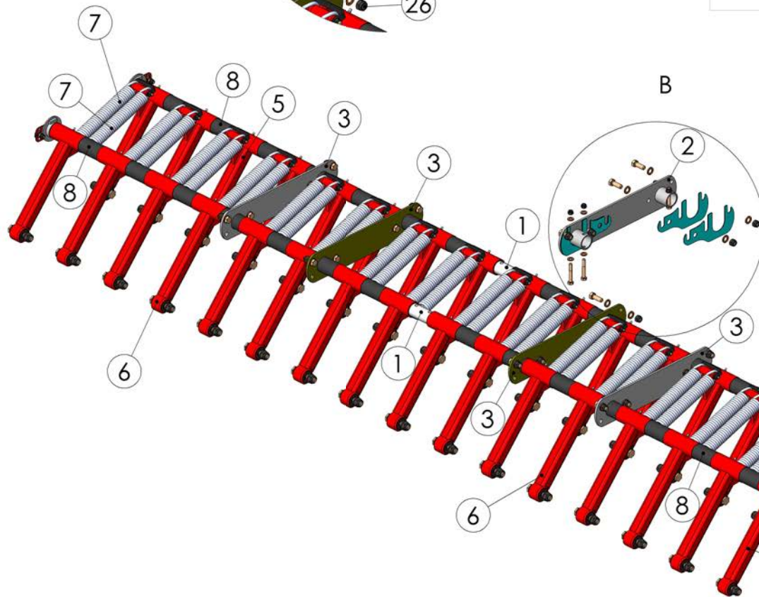
99532502 Parallel arms
