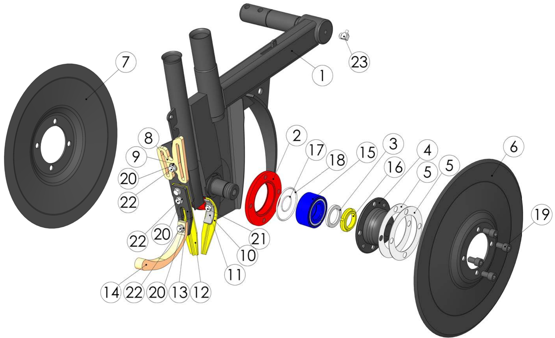
99562902 Front coultter
