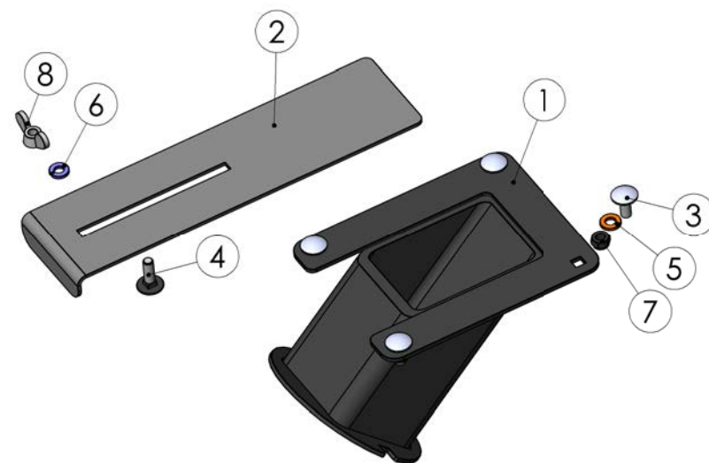
99309003 Valve
