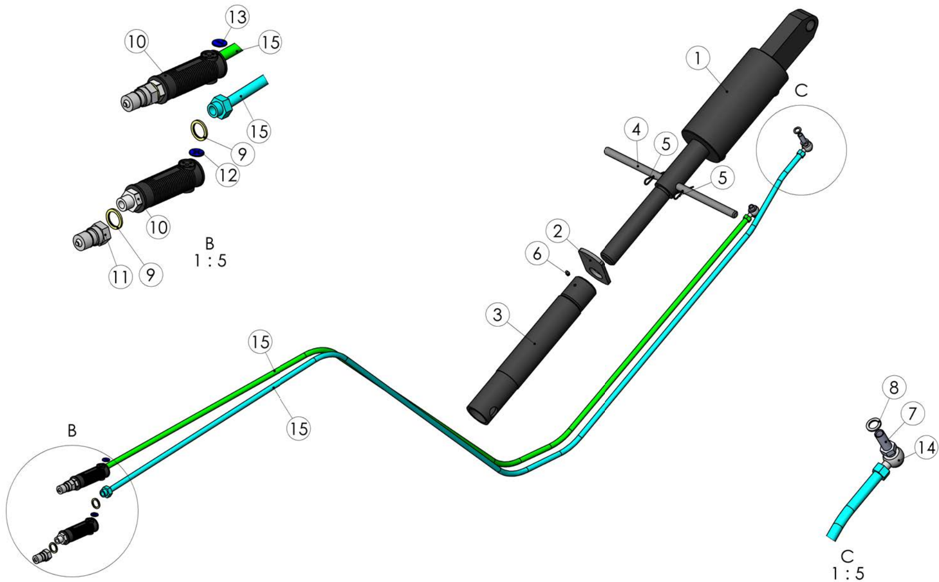
98635603 Cylinder
