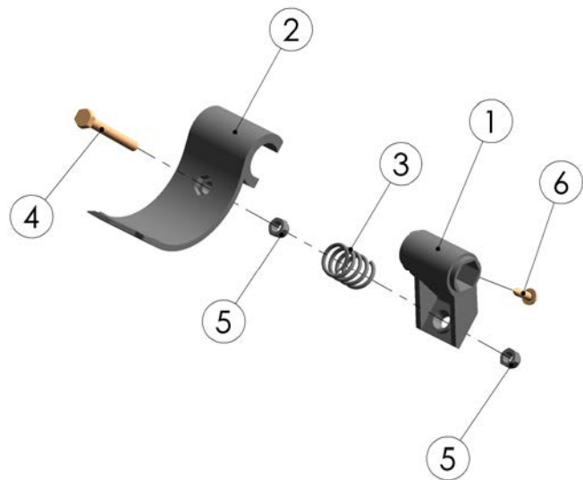
95524804 Bottom flap valve
