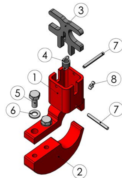
99236703 Governor
