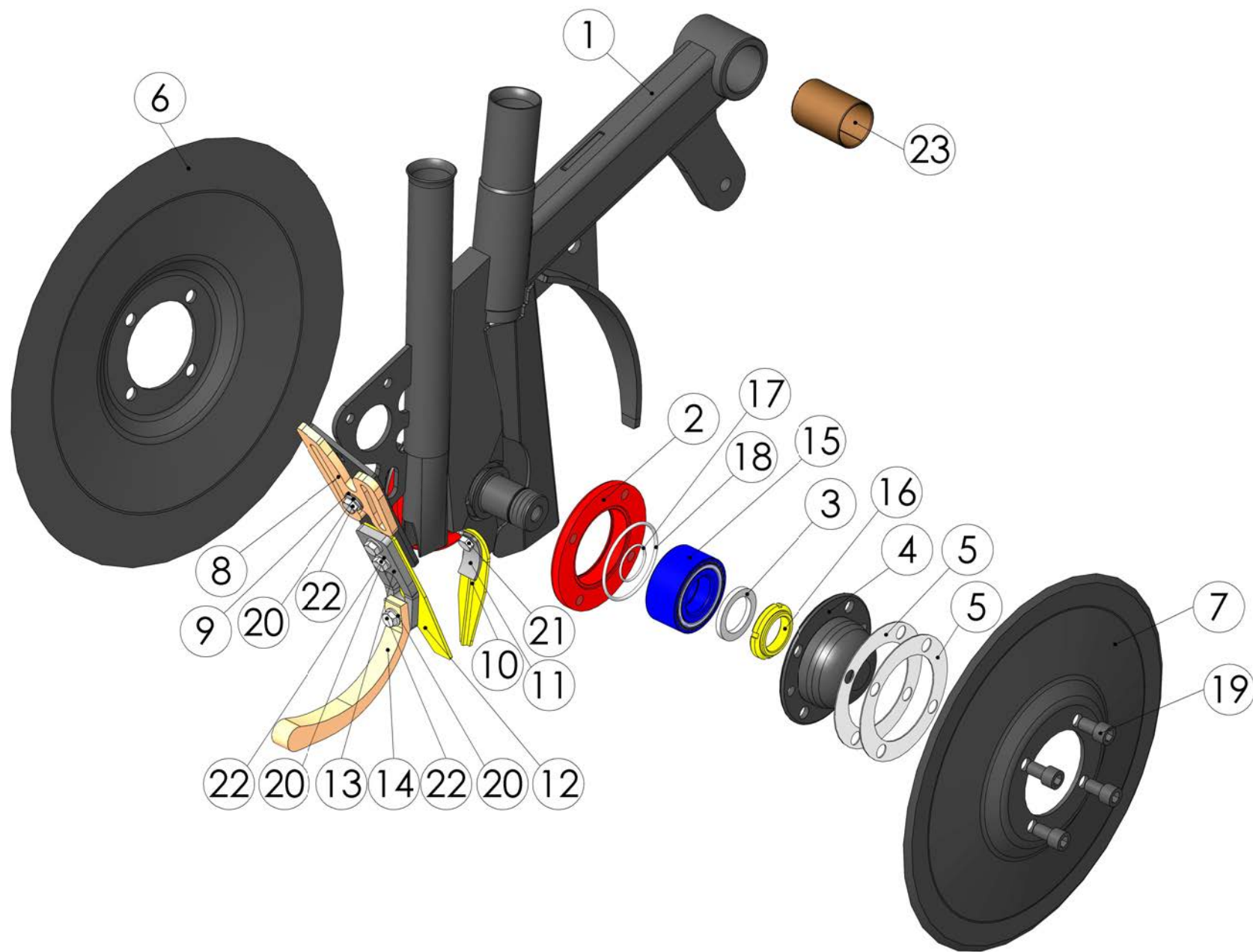
99563102 Back coultter
