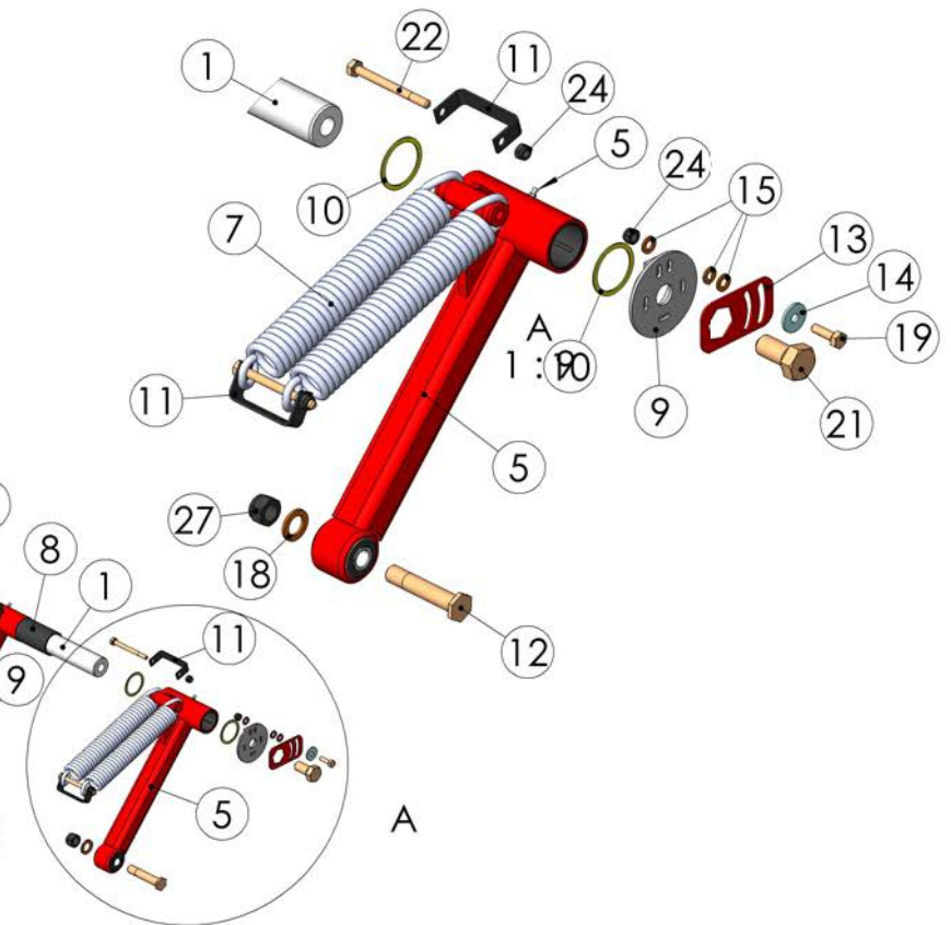
99296603 Front arm
