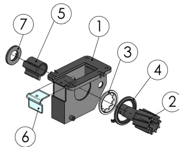
96202503 Feeding chamber, seed
