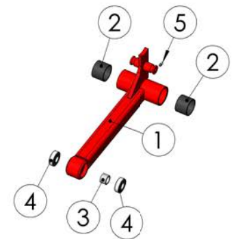
99323903 Rear arm
