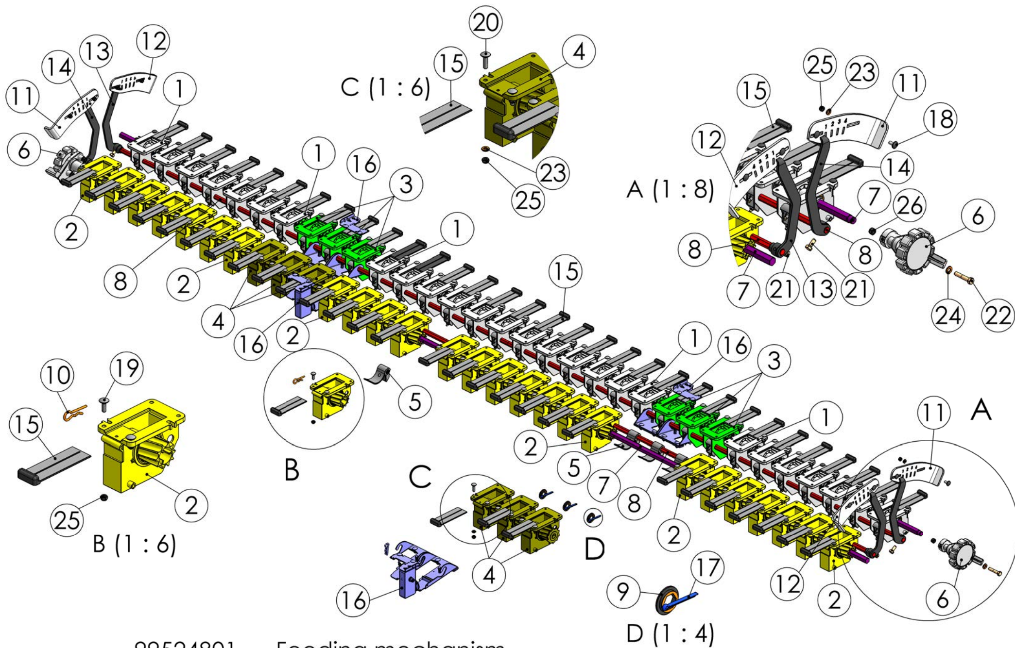
99524801 Feeding mechanism
