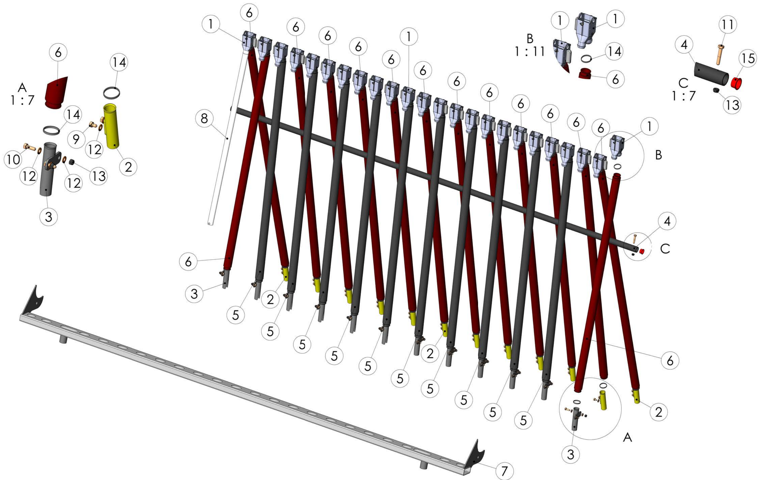
99519403 Hose start fertilizer
