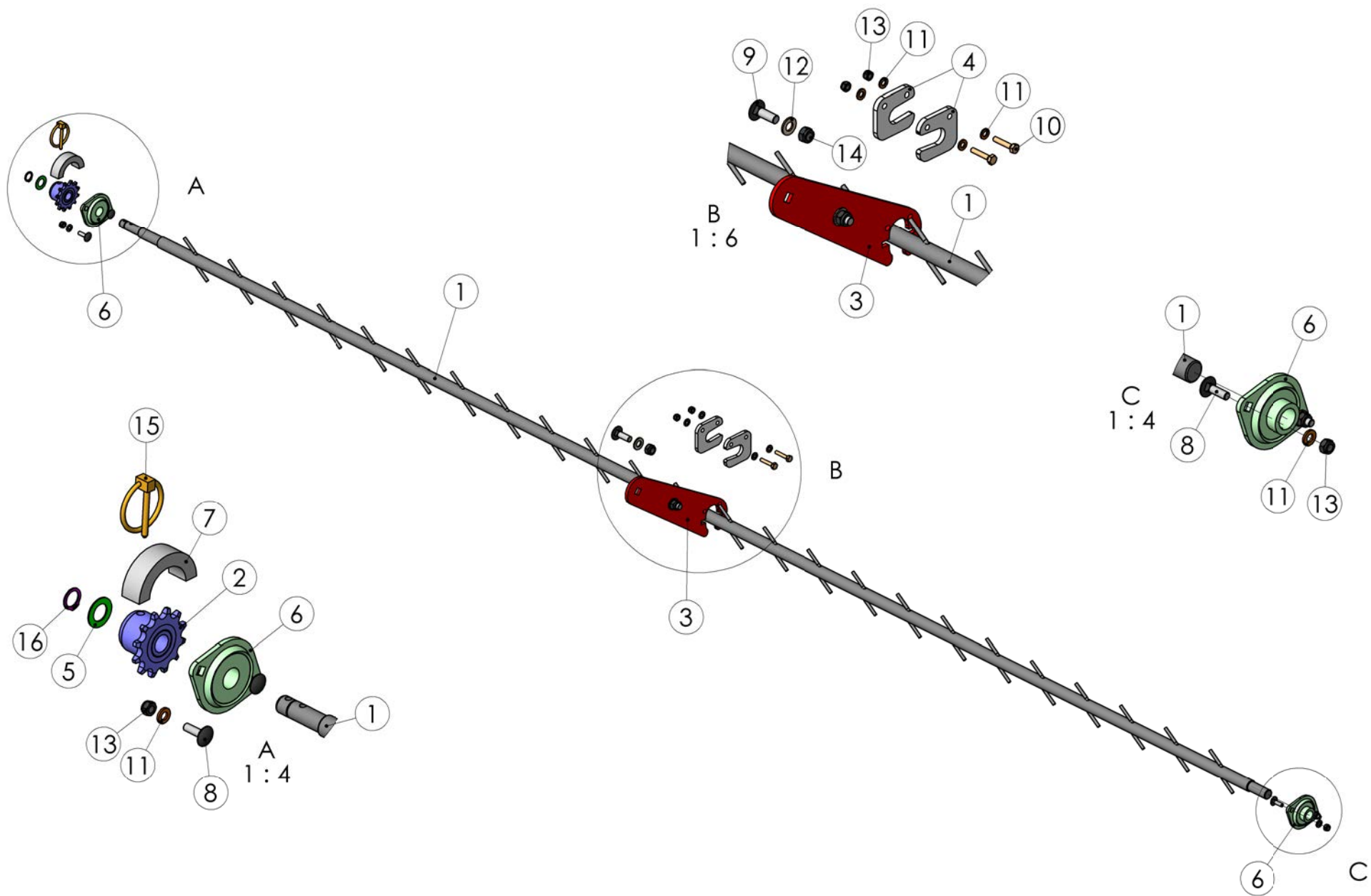
99545702 Mixer shaft grass seed
